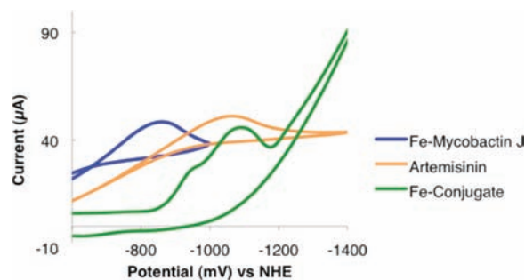
Figure 3. Cyclic voltammograms of Fe-loaded mycobactin J, artemisinin, and the Fe-loaded mycobactin–artemisinin conjugate. Conditions: glassy carbon working electrode; Pt wire auxiliary electrode; Ag/AgCl reference electrode; scan rate = 10 \text{ mV/s} ; [\text{NaClO}_4] = 100 \text{ mM} as the background electrolyte in 95% EtOH. [\text{Fe-mycobactin J}] = 3 \text{ mM} , E_{\text{cp}} = -856 \text{ mV vs NHE} ( 7 \mu\text{A}/\text{mM} ); [\text{artemisinin}] = 3 \text{ mM} , E_{\text{cp}} = -1063 \text{ mV vs NHE} ( 9 \mu\text{A}/\text{mM} ); [\text{Fe-mycobactin-artemisinin conjugate}] = 1.625 \text{ mM} , E_{\text{cp}} = -955 \text{ mV vs NHE} ( 18 \mu\text{A}/\text{mM} ), E_{\text{cp}} = -1090 \text{ mV vs NHE} ( 19 \mu\text{A}/\text{mM} ).
